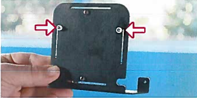
Figure 1 – Mounting Posts
