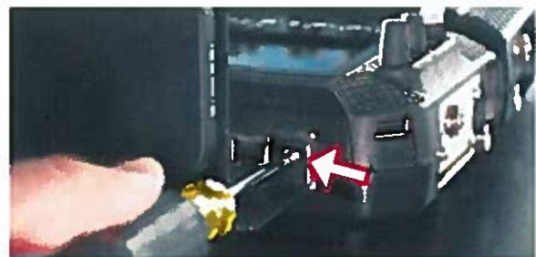
Figure 6 – Bracket Position
