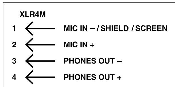
Figure 2. Headset connection pinout chart
